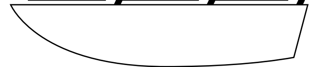
docker-machine
