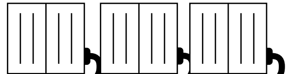
docker swarm
