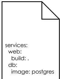
docker-compose.yml
